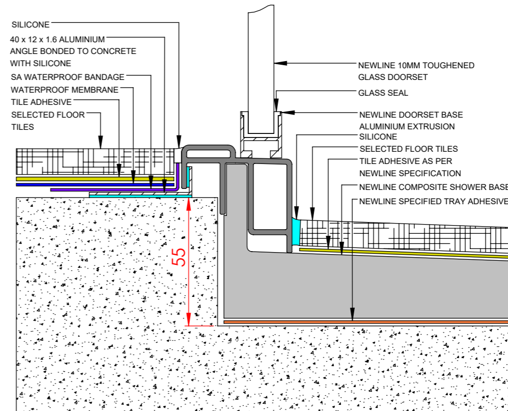
DRYFIT RECESSED TRAY SILL DETAIL
