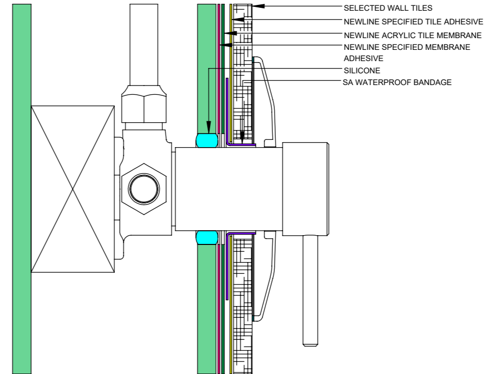
DRYFIT PIPE/MIXER PENETRATION DETAIL
