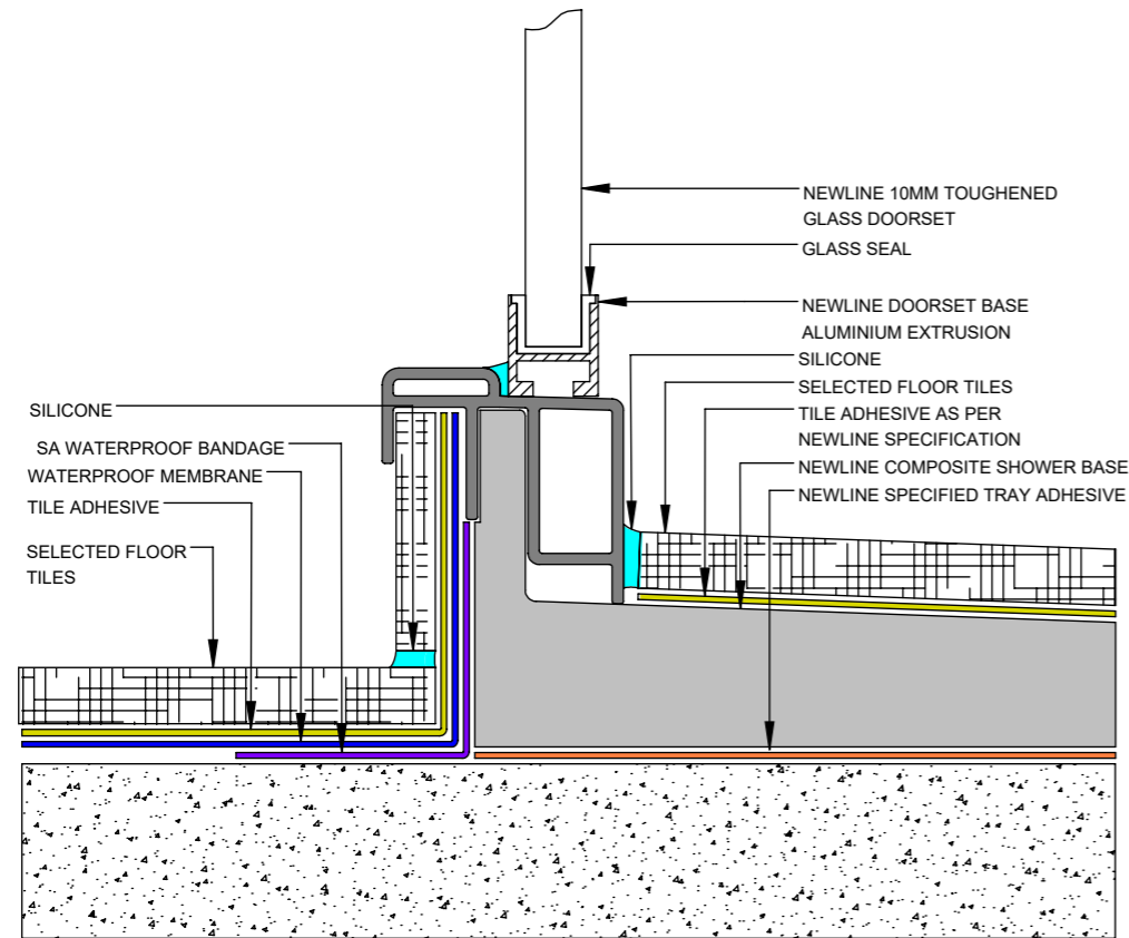
DRYFIT HOBBED TRAY SILL DETAIL
