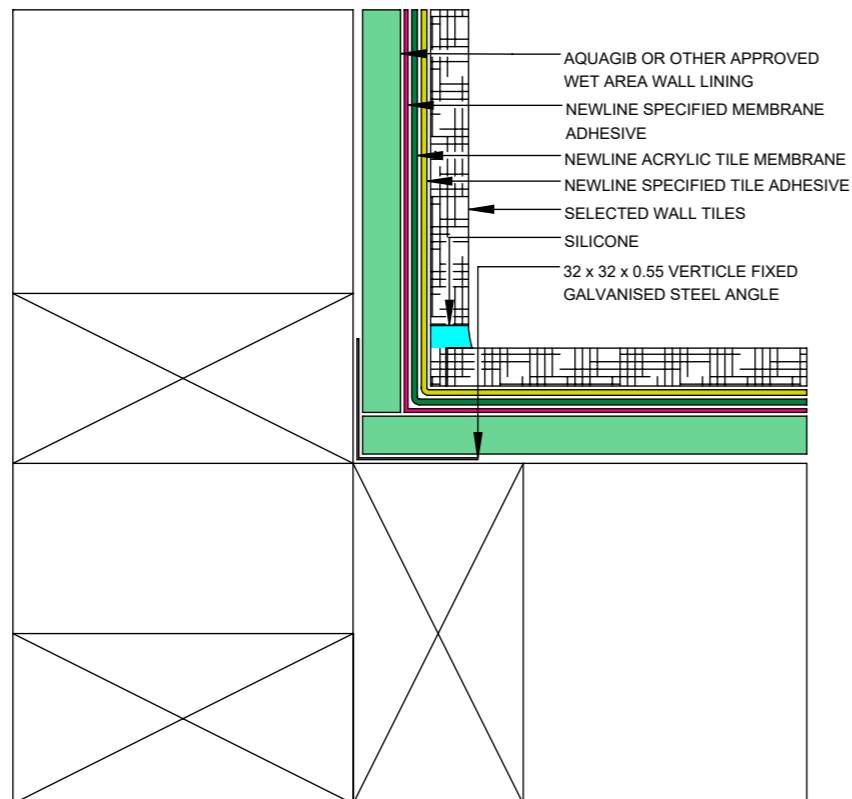
DRYFIT INTERNAL CORNER DETAIL
