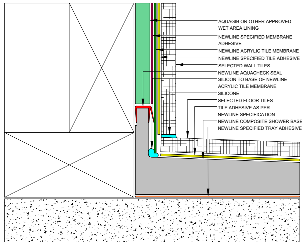
DRYFIT WALL/TRAY CROSS SECTION
