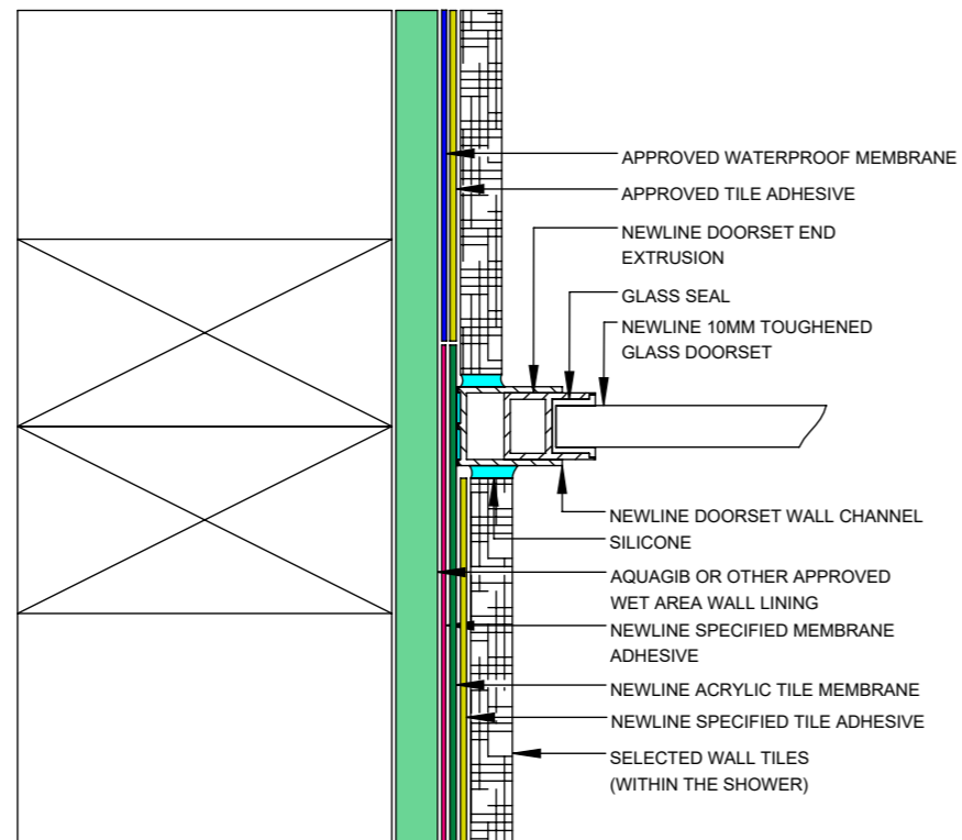
DRYFIT WALL CHANNEL DETAIL
