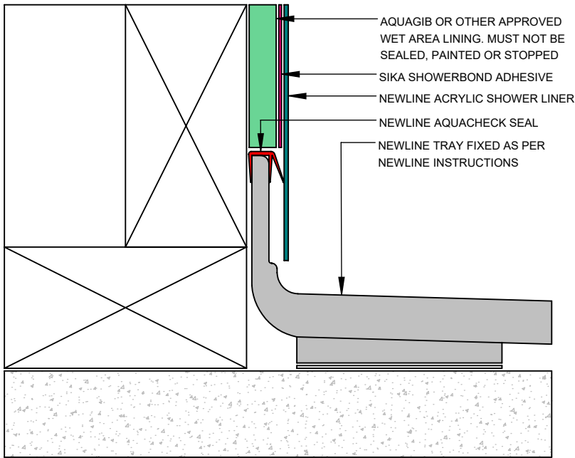
ACRYLIC LINER TRAY DETAIL
