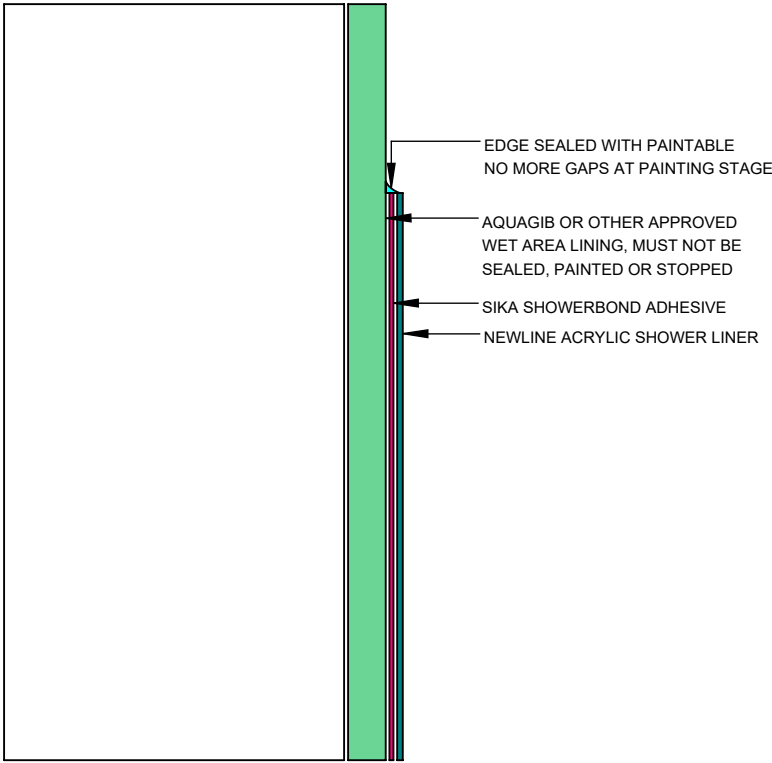
ACRYLIC LINER TOP OF WALL DETAIL
