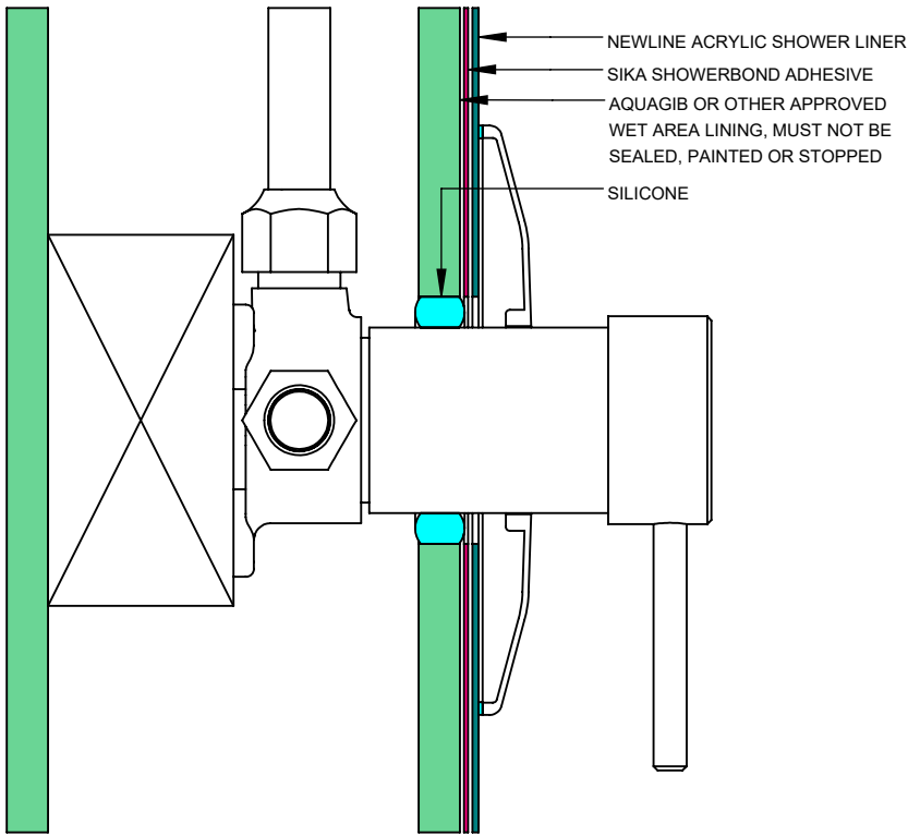
ACRYLIC LINER PIPE/MIXER PENETRATION DETAIL
