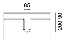
Drawer Cutout Detail (Top Drawer Only)
