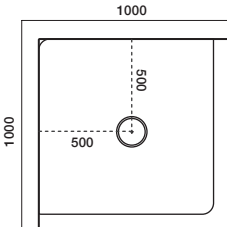
1000x1000 2-Sided Centre Waste
