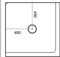
900x900 2-Sided Centre Waste
