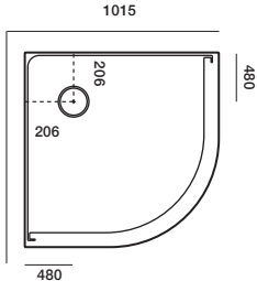
1015x1015 Curved Centre Waste
