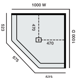
1000x1000 Neo RH Hobbed Centre Waste
