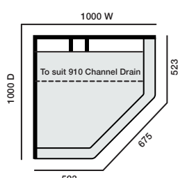
1000x1000 Neo LH Hobbed Channel
