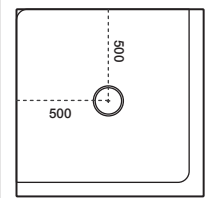
1000x1000 2-Sided Centre Waste
