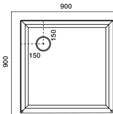
900x900 2-Sided Offset Waste
