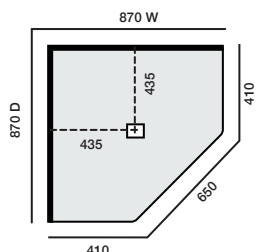
900x900 Neo LH or RH Recessed Centre Waste
