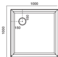
1000x1000 2-Sided Offset Waste
