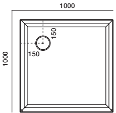
1000x1000 3-Sided Offset Waste
