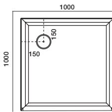
1000x1000 LH or RH
