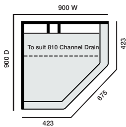
900x900 Neo LH Hobbed Channel
