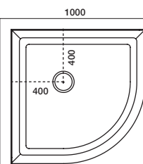
1000x1000 Curved Centre Waste
