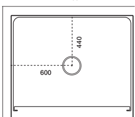
1200x915 3-Sided Centre Waste
