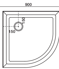
900x900 Curved Offset Waste
