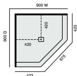
900x900 Neo LH or RH Hobbed Centre Waste
