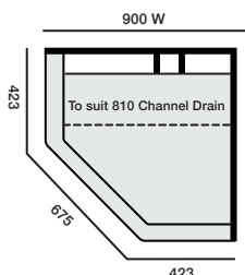
900x900 Neo RH Hobbed Channel
