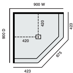
900x900 Neo LH Hobbed Centre Waste
