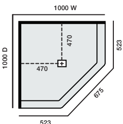
1000x1000 Neo LH Hobbed Centre Waste
