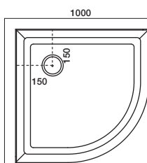
1000x1000 Curved Offset Waste
