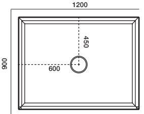
1200x900 3-Sided Centre Waste
