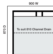
900x900 3-Sided Recessed Channel
