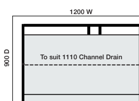
1200x900 3-Sided Hobbed Channel
