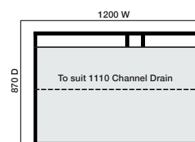
1200x900 3-Sided Recessed Channel
