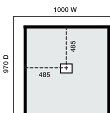
1000x1000 3-Sided Recessed Centre Waste
