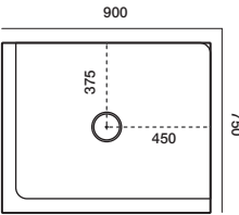
900x750 2-Sided RH Centre Waste
