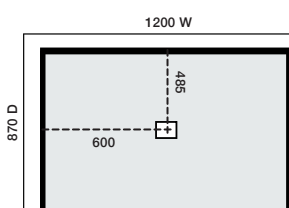
1200x900 3-Sided Recessed Centre Waste
