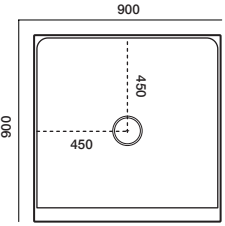
900x900 3-Sided Centre Waste
