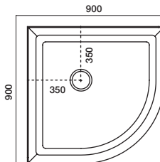
900x900 Curved Centre Waste
