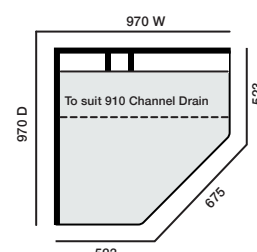
1000x1000 Neo LH Recessed Channel
