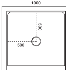
1000x1000 3-Sided Centre Waste
