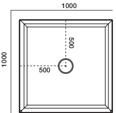
1000x1000 3-Sided Centre Waste
