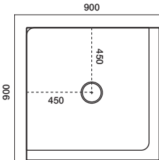
900x900 2-Sided Centre Waste
