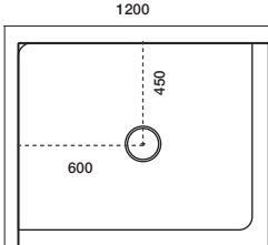
1200x900 2-Sided LH Centre Waste
