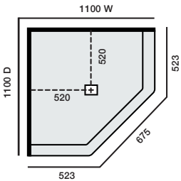
1100x1100 Neo LH Hobbed Centre Waste
