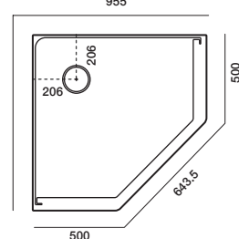
955x955 Neo Offset Waste
