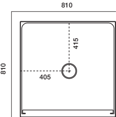
810x810 3-Sided Centre Waste
