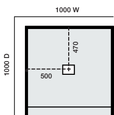
1000x1000 3-Sided Hobbed Centre Waste
