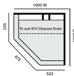
1000x1000 Neo RH Hobbed Channel
