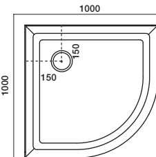
1000x1000 Curved Offset Waste
