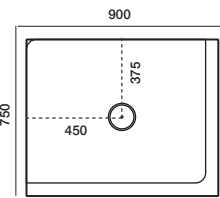
900x750 2-Sided LH Centre Waste
