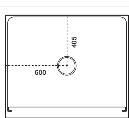
1200x800 3-Sided Centre Waste
