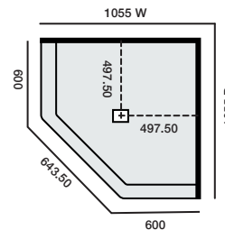
1055x1055 Neo RH Hobbed Centre Waste
