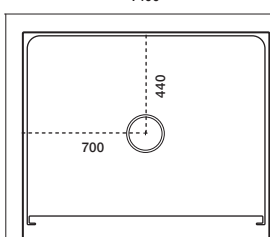
1400x915 3-Sided Centre Waste
