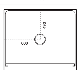
1200x1000 3-Sided Centre Waste
