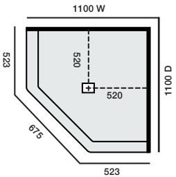
1100x1100 Neo RH Hobbed Centre Waste
