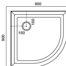
900x900 Curved Offset Waste
