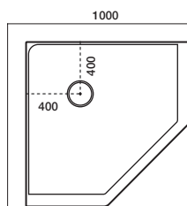
1000x1000 Neo Centre Waste
