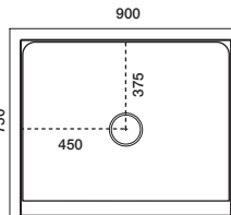
950x750 3-Sided Centre Waste
