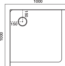
1000x1000 2-Sided Offset Waste
