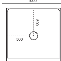
1000x1000 3-Sided Centre Waste
