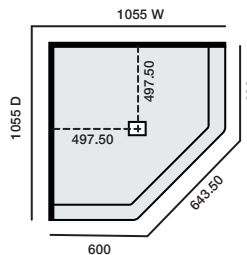
1055x1055 Neo LH Hobbed Centre Waste
