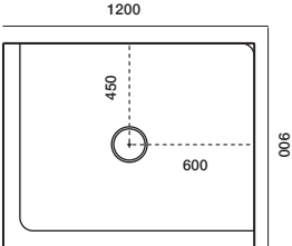
1200x900 2-Sided RH Centre Waste
