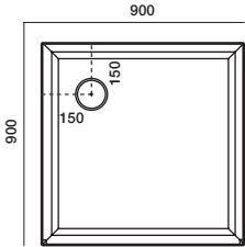
900x900 3-Sided Offset Waste
