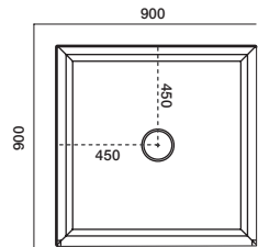
900x900 2-Sided Centre Waste
