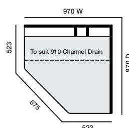
1000x1000 Neo RH Recessed Channel
